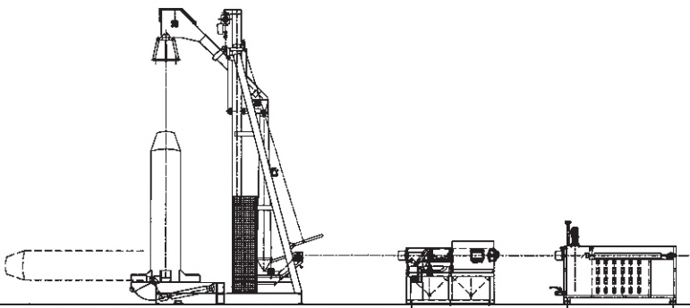
Vertical pay-off model POH 65
